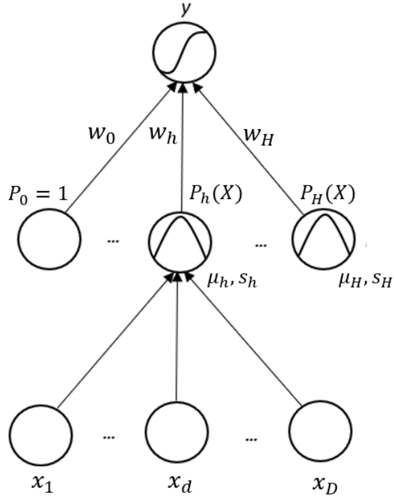
Figure 2.1: Standard Architecture of an RBF Network with H Gaussian Kernels (Alpaydin, 2004)
