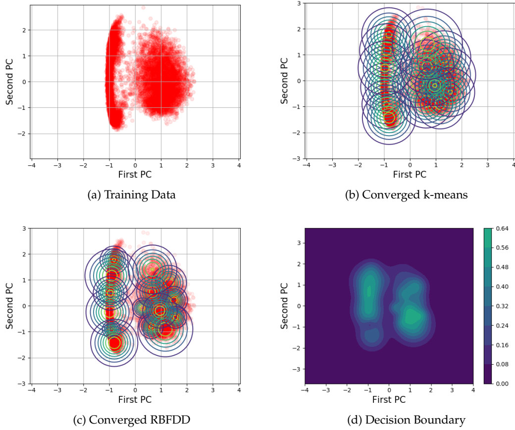
Figure 4.2: Considering images of digits 0 and 1 from the MNIST dataset as class normal instances for training and using the first two principal components, we have the visualisations of the transformed training data after applying PCA in red circles, the Gaussians after k-means pre-training, trained RBFDD network, and the decision surface of the trained RBFDD network.
