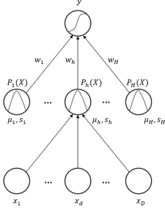
Figure 4.1: The RBFDD network.
