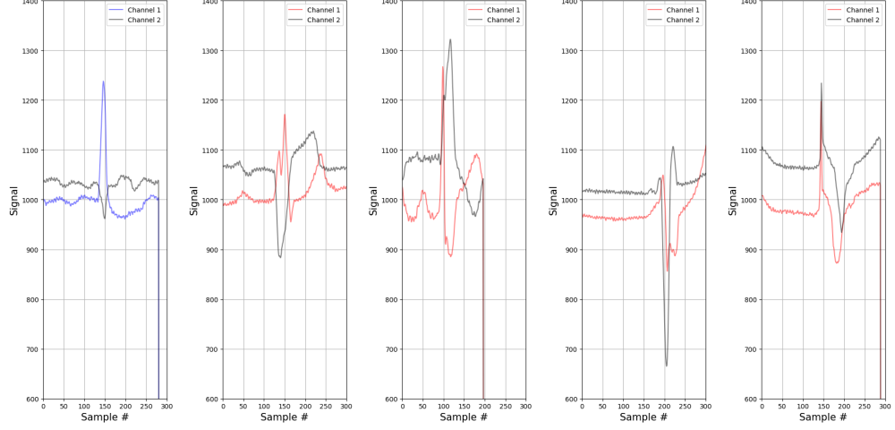
Figure 3.2: Individual heart-beat samples (from left to right) from normal, left bundle branch block beat, right bundle branch block beat, premature ventricular contraction, and paced beat classes
