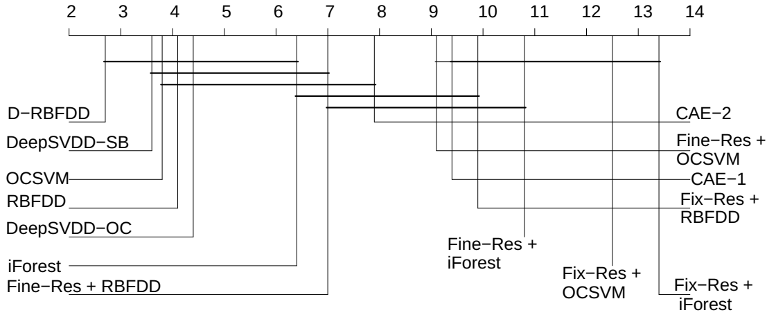
(a) On cases of MNIST and Fashion MNIST datasets
