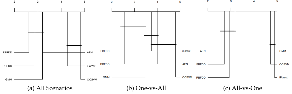
Figure 5.4: Critical difference plots from Friedman’s test with Finner p -value correction with significance level \alpha = 0.05
