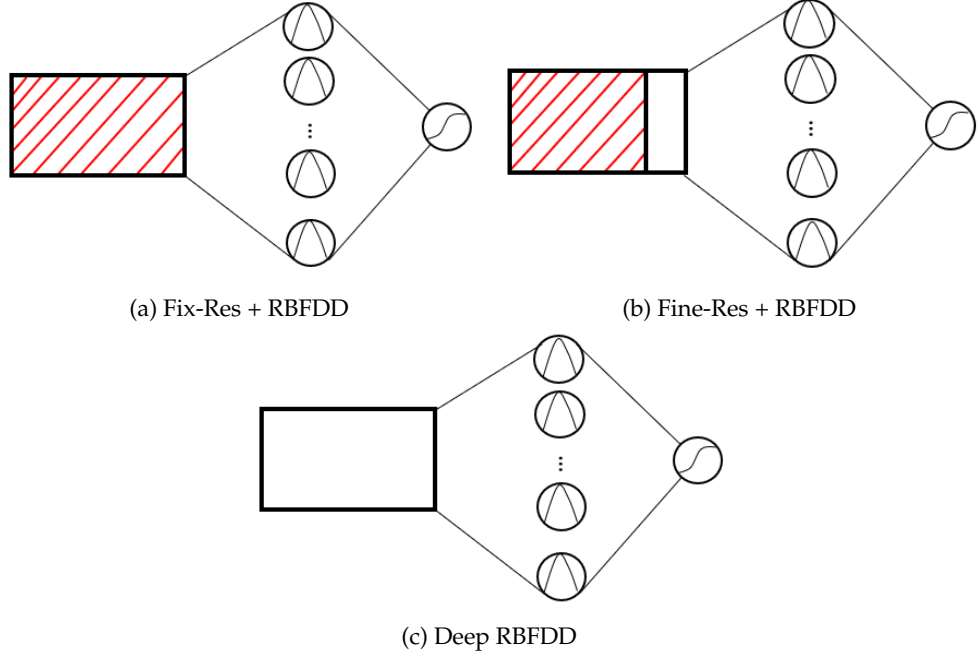
Figure 6.1: Three approaches to deepening RBFDD networks. The red lines highlight the fixed portion of each model.
