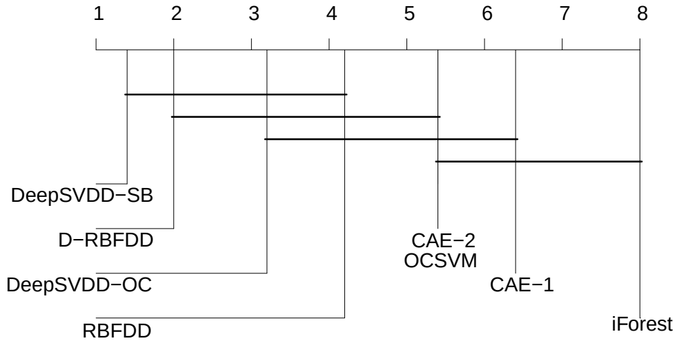
(b) On cases of MIT-BIH Arrhythmia dataset
