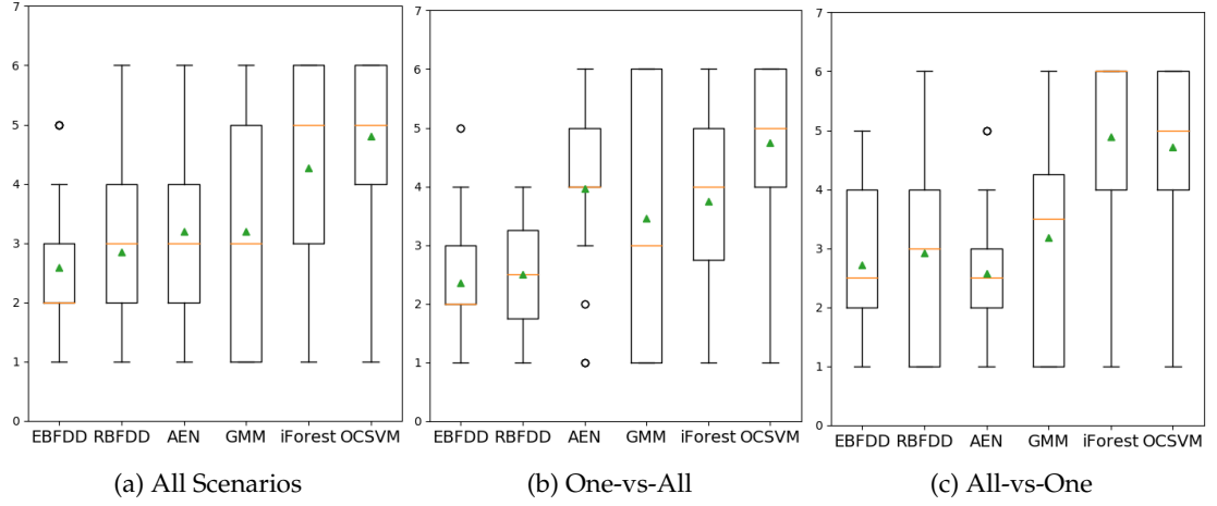
Figure 5.3: The average rank of the algorithms across the experiments. On each box plot the median ranks are shown via the horizontal orange lines and the mean ranks are shown using green triangles.
