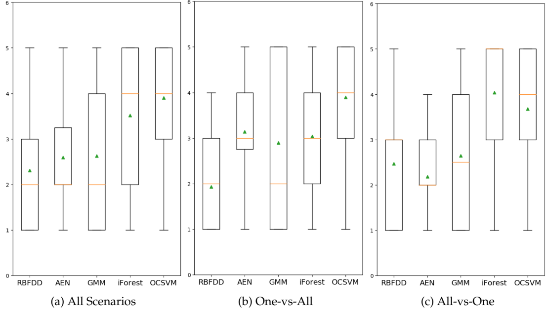
Figure 4.4: The average rank of the algorithms across the experiments. On each box plot the median ranks are shown via the horizontal orange lines and the mean ranks are shown using green triangles.
