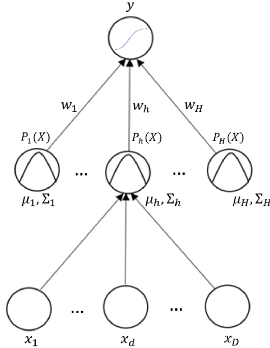
Figure 5.1: The Architecture of the EBFDD network.
