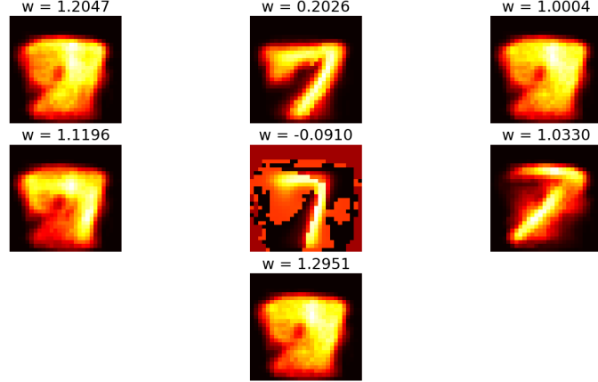
Figure 4.3: The centres of 7 Gaussians of a trained RBFDD network with their corresponding learned weights, where the normal class consists of images of digit 7 from the MNIST dataset.
