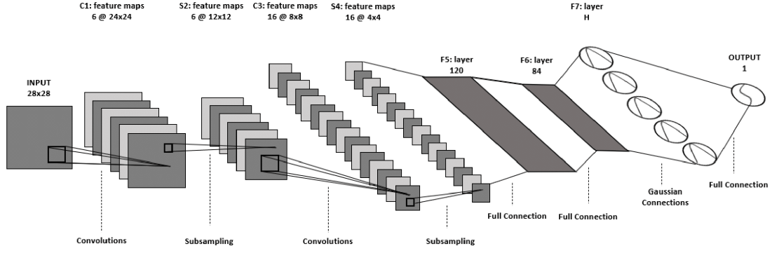
Figure 6.2: The Deep RBFDD Anomaly Detector
