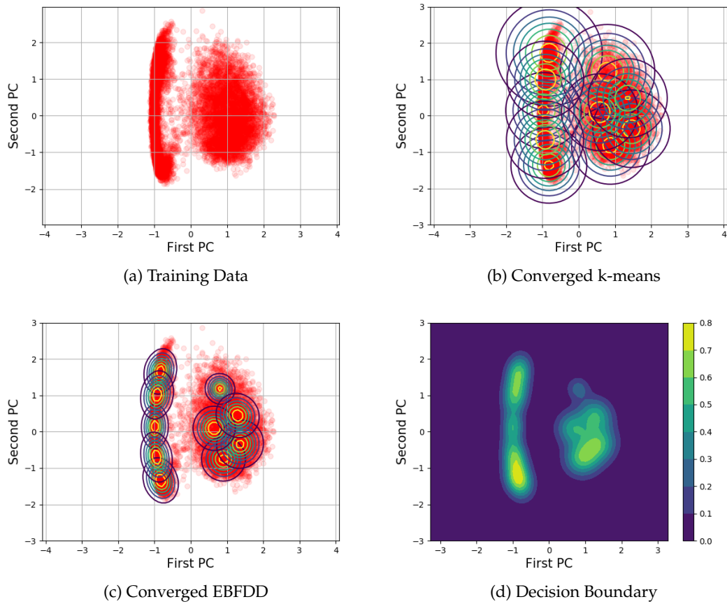
Figure 5.2: Considering images of both digits 0 and 1 from the MNIST dataset as class normal instances for training and using the first two principal components, we have the visualisations of the transformed training data after applying PCA in red circles, the Gaussians after k-means pre-training, trained EBFDD network, and the decision surface of the trained EBFDD network.
