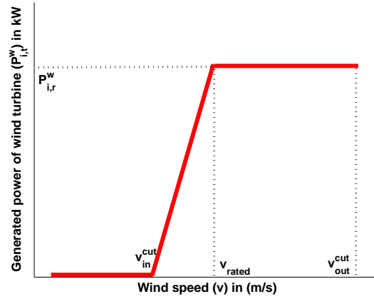
Fig. 2. The idealized power curve of a wind turbine
