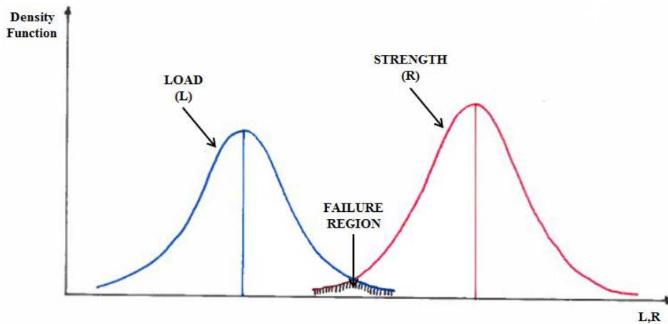
Figure 4. Frequency distribution of strength R and Loads L (Adapted from Ayyub and Assakkaf 2000)
