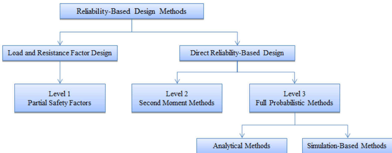
Figure 3. Levels of probability procedures for reliability-based design
