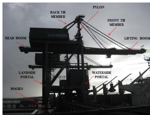
Figure 1. Ship unloader elements: Lower (Bogies, waterside portal, landside portal, hopper and diagonal brace) and Upper Substructures (Lifting boom, rear boom, front tie member, back tie member and pylon)
