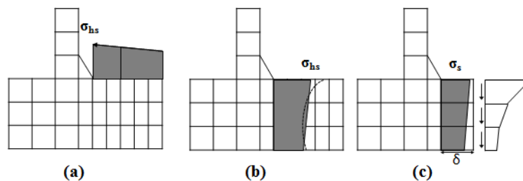
Figure 2. Evaluation of structural stress at weld toe by (a) surface stress extrapolation; (b) linearization over plate thickness and (c) equilibrium with stresses at distance \delta . (Adapted from Fricke and Kahl 2005)
