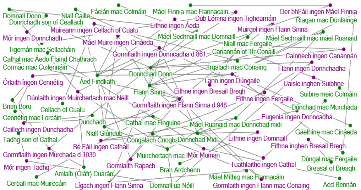
Fig. 1 Purple nodes represent queens and green nodes represent kings.
