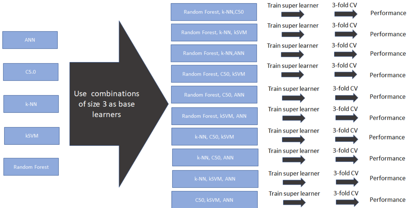
Fig. 3. Experiment 3 - Evaluation of prediction performance of the stacked classifier with default parameters
