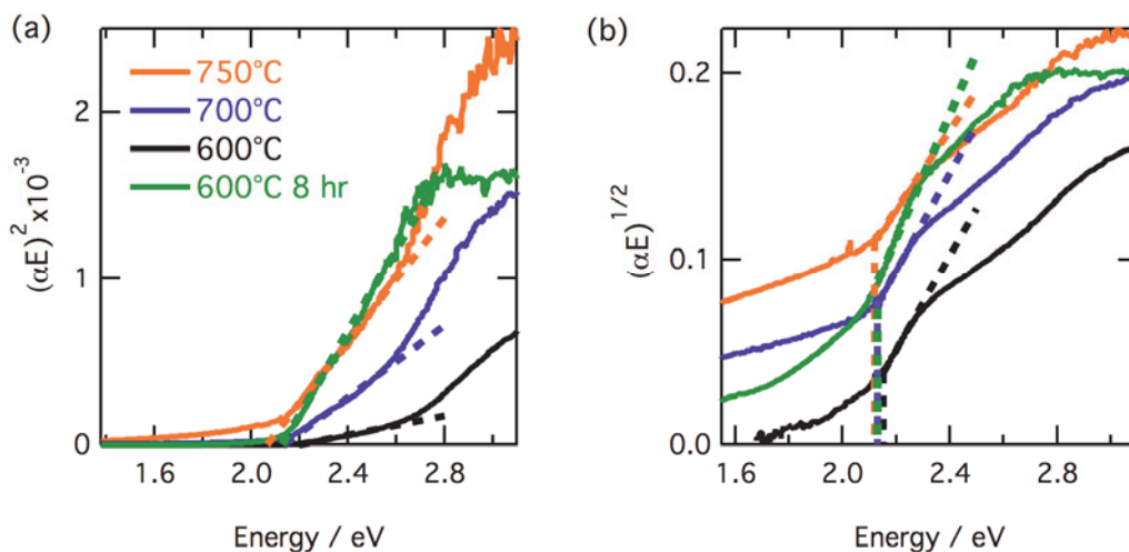
Figure S4: Tauc analysis assuming a (a) direct transitions and (b) indirect transitions of hematite samples annealed for 5 minutes at 600, 700, and 750 °C in comparison to a sample annealed at 600 °C for 8 hours.
