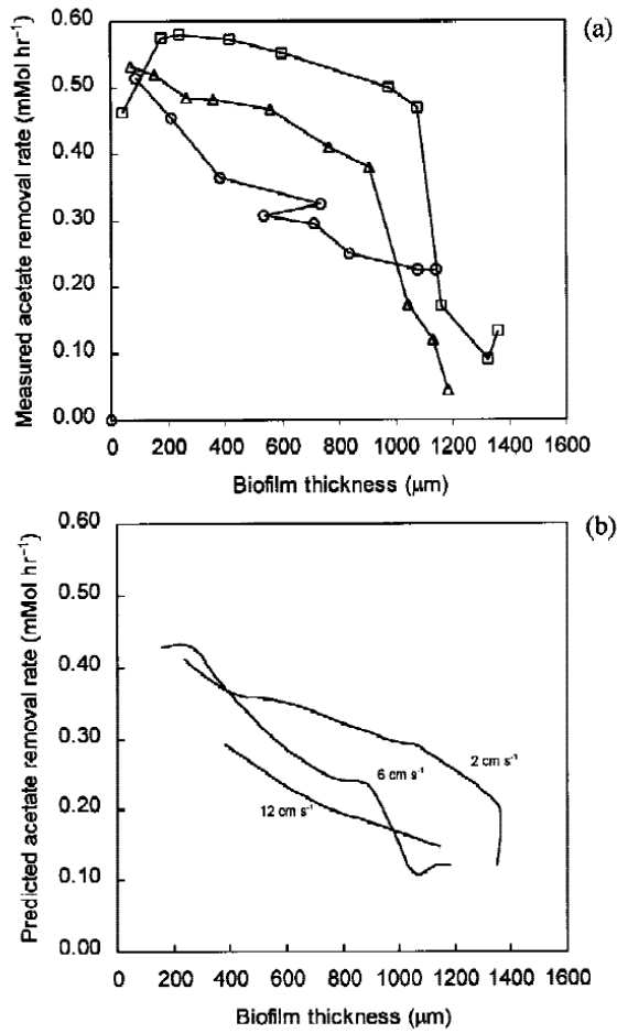
Figure 10. (a) Experimentally observed acetate removal rates plotted against biofilm thickness for flow velocities of 2 (□), 6 (△), and 12 cm s -1 (○). Continuous lines represent trends through the data. (b) Model-predicted values of the acetate removal rates plotted against biofilm thickness.
