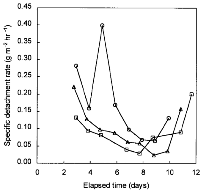
Figure 5. Specific biomass detachment rates during development of biofilms for flow velocities of 2 ( \square ), 6 ( \triangle ), and 12 \text{cm s}^{-1} ( \circ ).
