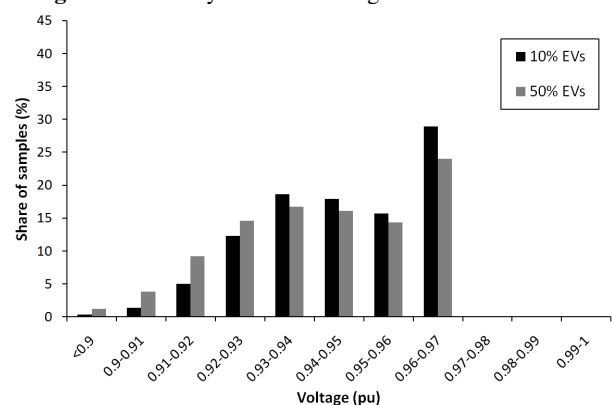
Fig. 6 - Probability of CPOC voltages for winter scenario
