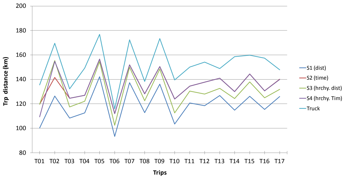
Figure 3: Travelling distance per route under different scenarios.
