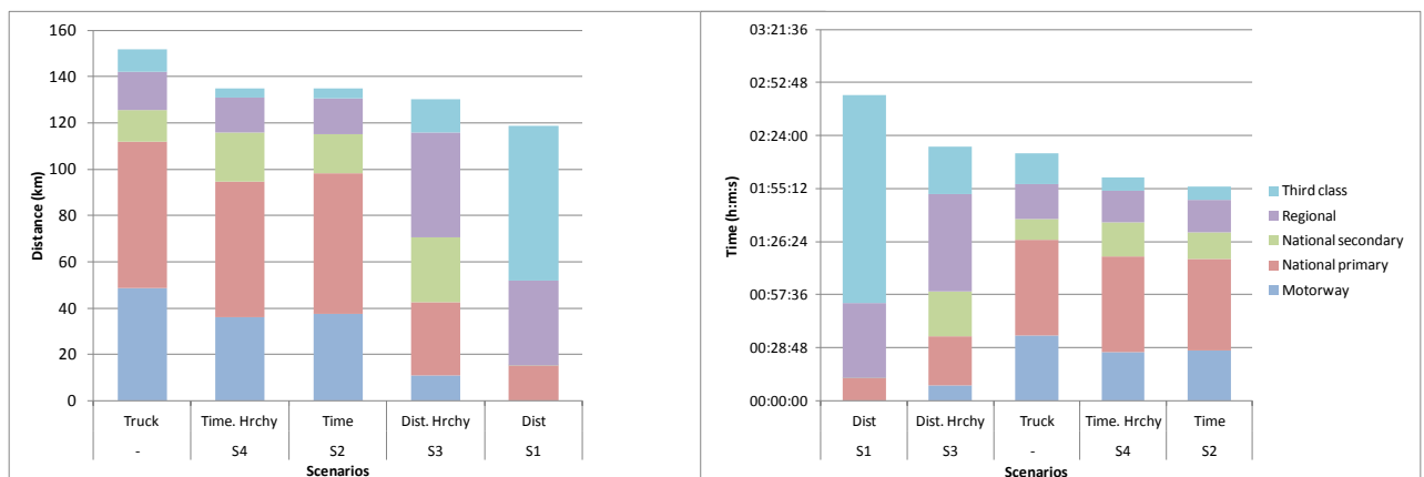
Figure 5: Different proportions of road types by routes under different scenarios.
