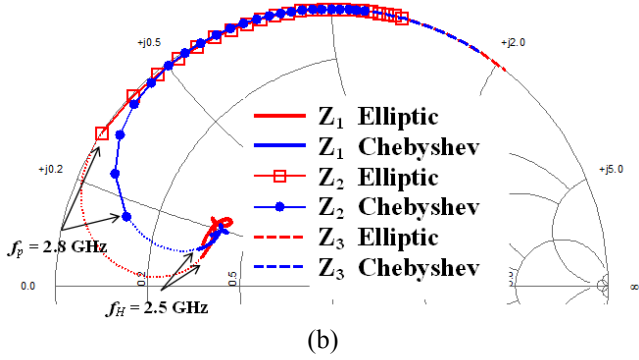
Fig. 8. Comparison between modified elliptic and Chebyshev LPF MNs. (a) Forward transfer function S_{21} and input return loss S_{11} . (b) Impedance trajectories from the fundamental to the third harmonic.
