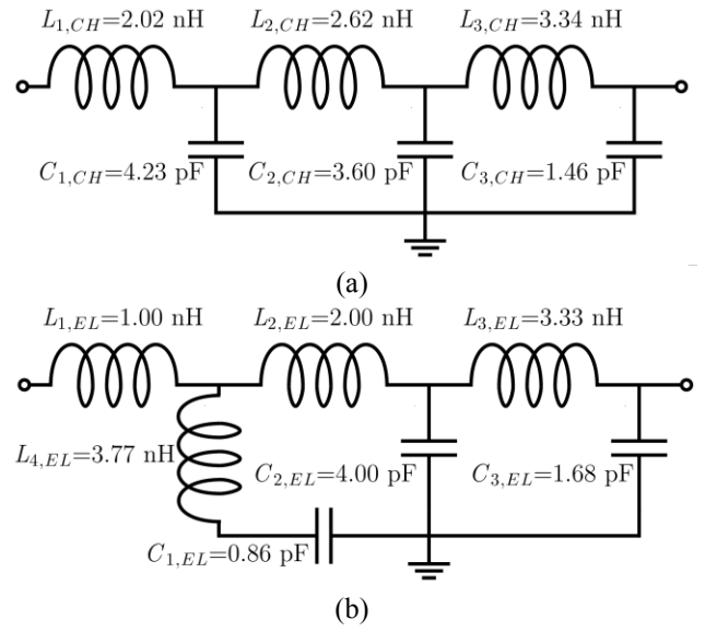
Fig. 7. LC prototypes. (a) Prototype of Chebyshev LPF MN. (b) Prototype of modified elliptic LPF MN.
