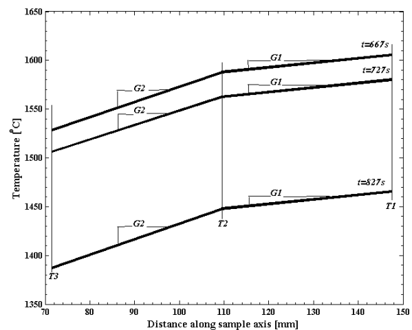
Figure 3. Schematic of Power-down technique
