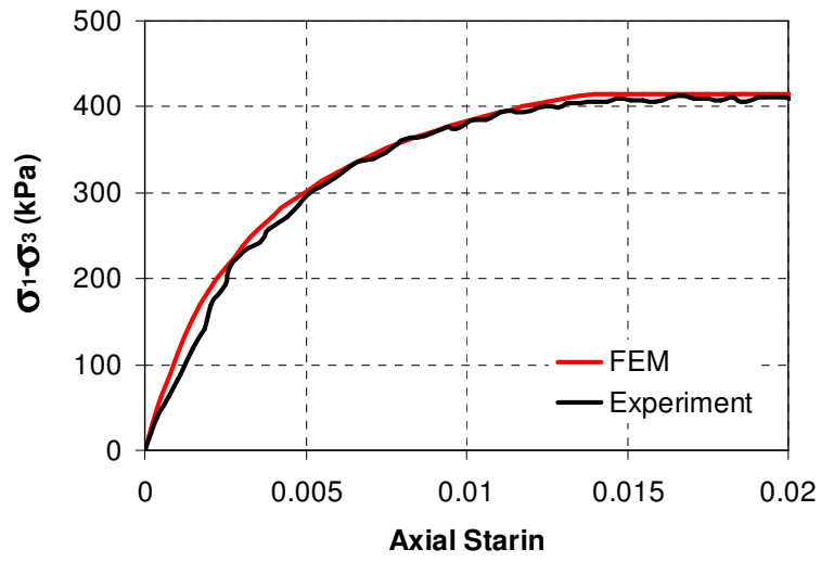
Fig. 5. Comparison of experimental and FEM triaxial test
