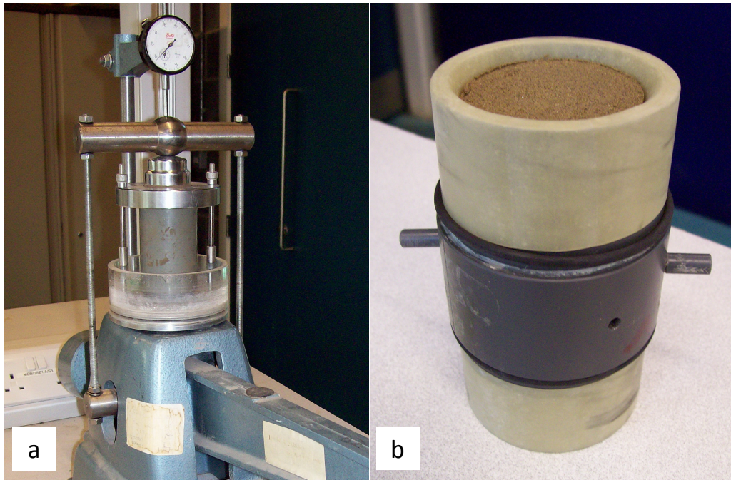
Fig. 3. Triaxial sample preparation (Tolooiyan, 2010)
