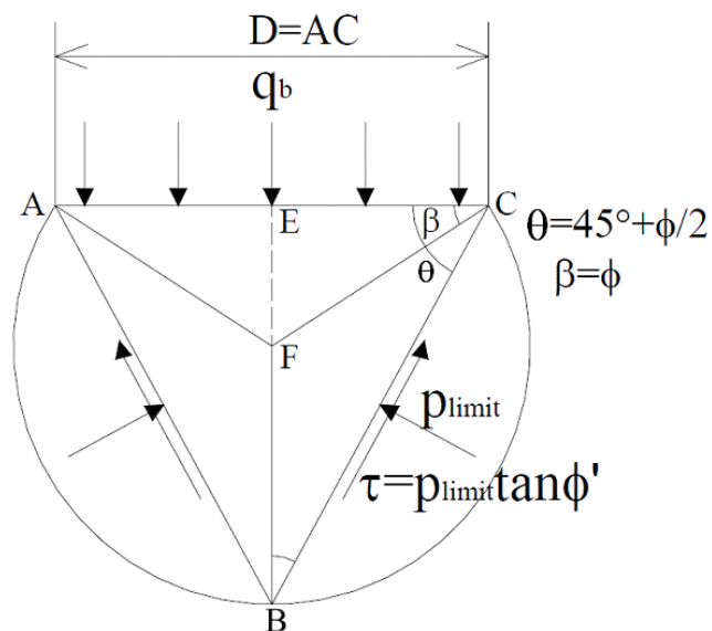
Fig. 1. Randolph et al. (1994) relationship between tip resistance q_b and cavity limit pressures P_{\text{limit}}
