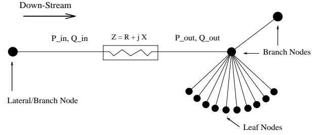
Figure 7: Typical lossy line
