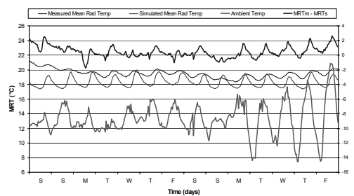
Figure 4: ESPr Validation: Mean Radiant Temperature.
