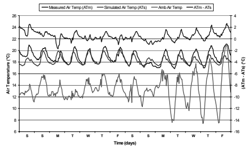
Figure 3: ESPr Validation: Air Temperature.
