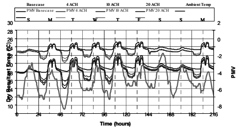
Figure 6: Dry Resultant Temperatures and ACHs (Model 3, Internal Gains = 32W/m 2 ).
