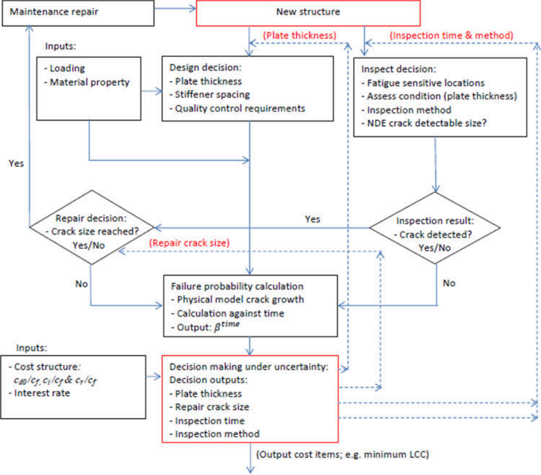
Figure 9. Illustration of risk-informed decision support approach for holistic fatigue management
