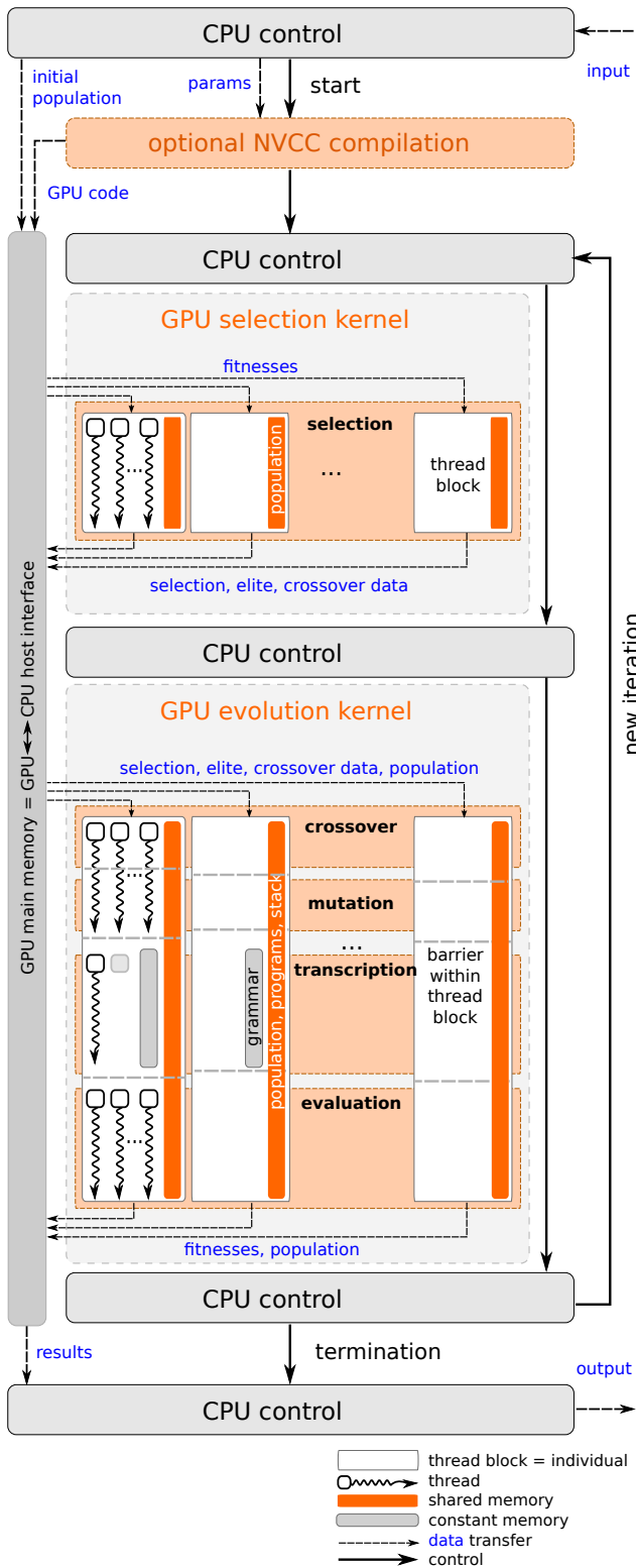
Figure 4: Grammatical evolution running on GPU
