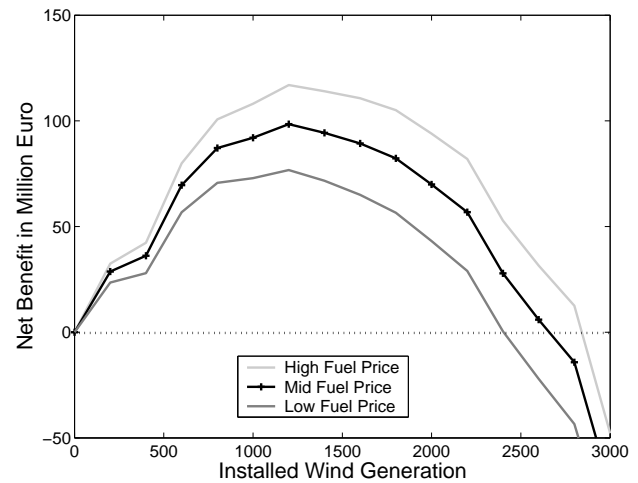
Fig. 8. Net benefits of wind generation with three fuel price scenarios
