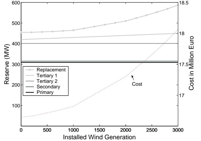
Fig. 2. Reserve requirements with increasing wind generation
