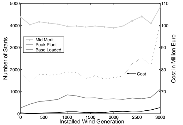
Fig. 3. Start-ups of conventional generation with increasing wind penetration
