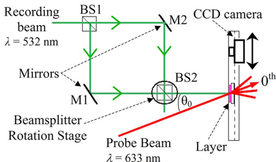
Fig. 1. (Color online) Setup for adjusting period and recording grating.
