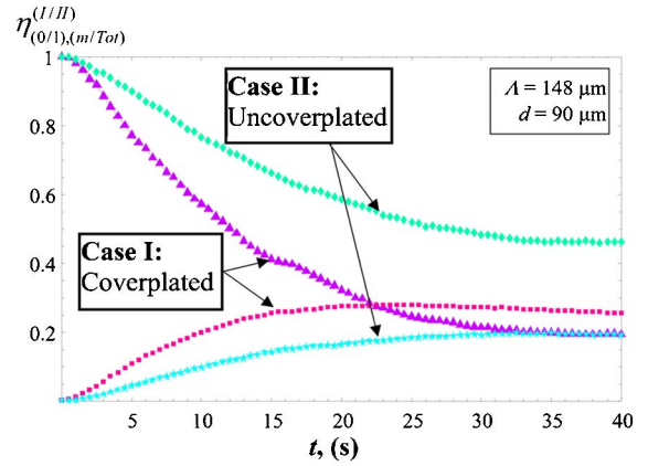
Fig. 6. (Color online) Evolution of the zeroth and first diffraction orders for Cases I and II where the recording intensity is 0.4 \text{ mW/cm}^2 .
